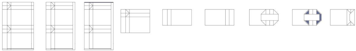
Automatic Feeding Top Folding Edge Gluing Edge Pasting Gusset formation Turn around and Flip over Bottom folding Gluing Bottom sealing
